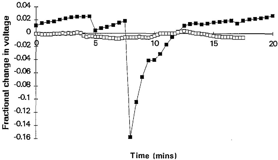
Figure 4. A comparison of the single best and worst baseline drift characteristics from this series of experiments: normalized mean voltage change (ratio) against time. ■, worst baseline drift; □, best baseline drift.
