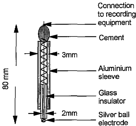
Figure 3. The construction of the spring-loaded electrodes used on the rabbit brain.
