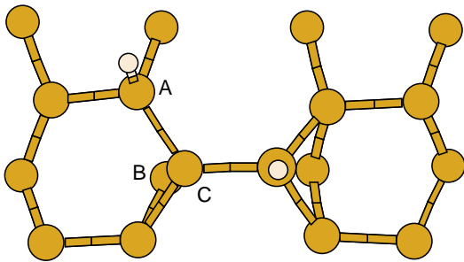
FIG. 2: The structure of the meta-stable state which provides a low energy pathway for dehydrogenation. The diffusing hydrogen is bonded to a substrate dimer (A), which has broken one bond to a second-layer silicon (B). The ad-dimer (C) is now partly clean, and has formed a bond to the second-layer silicon (B) left by the substrate dimer.
