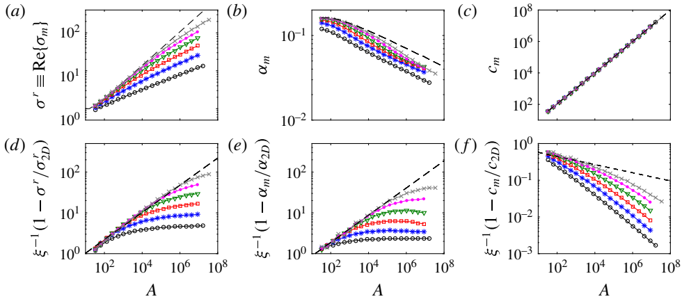
FIGURE 6. (Colour online) Data (dots) as a function of A , for different aspect ratios \xi . ( a – c ) The maximum growth rate \sigma^r \equiv \text{Re}\{\sigma_m\} , with the corresponding vertical wavenumber \alpha_m and the propagation speed c_m , together with the two-dimensional results (black dashed lines), which exhibit asymptotic scalings of \text{Re}\{\sigma_{2D}\} \sim A^{4/9} , \alpha_{2D} \sim A^{-1/9} and c_{2D} \sim A as A \rightarrow \infty . ( d – f ) The relative deviation from the two-dimensional results, scaled by the aspect ratio \xi , for the same three quantities. The dashed lines show the asymptotic predictions for \xi \rightarrow 0 taken from (4.13) (see asymptotic analysis in § 4). The quantities deviate from the asymptotic predictions as A \rightarrow \infty , as discussed in § 4.3. The different symbols correspond to \xi = 1/5 (black circles), \xi = 1/10 (blue stars), \xi = 1/20 (red squares), \xi = 1/40 (green triangles), \xi = 1/80 (pink dots) and \xi = 1/160 (grey crosses).
