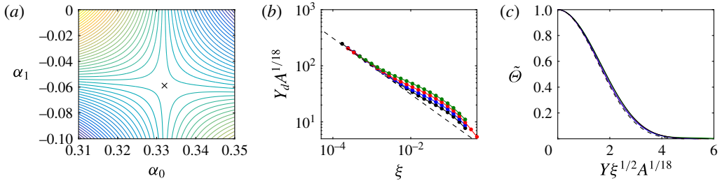
FIGURE 9. (Colour online) (a) Contours of the correction to the growth rate \text{Re}\{S_1\} as a function of the wavenumbers \alpha_0 and \alpha_1 , as defined in appendix A. The saddle point (\alpha_0, \alpha_1) = (0.332, -0.059) is marked by a cross. (b) The width Y_d of the profiles in the y -direction, as defined in figure 8(b), scaled by A^{-1/18} and compared with the predicted width from the asymptotic analysis (4.12) (dashed line). (c) Temperature profiles in the Y -direction for \xi = 2^{-11} , as in figure 8(b), scaled by A^{-1/18} and compared with the Gaussian asymptotic prediction in (4.12) (dashed). In (b) and (c), the colours correspond to A = 2^{11} (black), A = 2^{14} (blue), A = 2^{17} (red) and A = 2^{20} (green).
