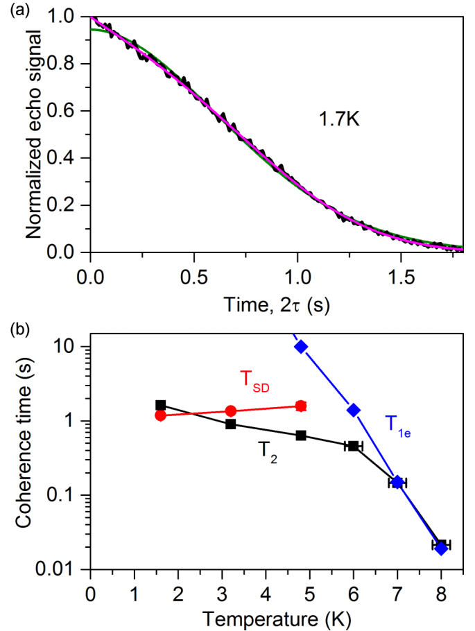
FIG. 1. (a) Nuclear spin Hahn echo decays for neutral ^{31}\text{P} donors in natural silicon ( f = 4.7\% ) at 1.7 K with magnetic field ( \sim 0.35 T) oriented along [001]. The pink curve is a fit of the data using Eq. (1). The green curve is a fit to \exp[-(2\tau/T_{\text{SD}})^n] demonstrating that using only one exponential term does not provide a good fit. A detailed comparison of the two fits for all four samples used in this work is presented in the Supplemental Material [24]. (b) Temperature dependencies of ^{31}\text{P} nuclear spin T_2 and T_{\text{SD}} (black squares and red circles, respectively) and electron spin T_{1e} times (blue diamonds) for neutral phosphorus donors in natural silicon. Vertical error bars in (b) are smaller than their symbols.
