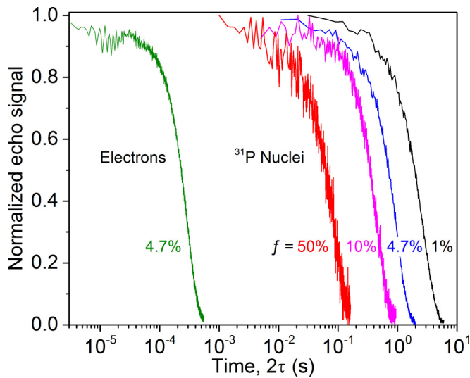
FIG. 2. ^{31}\text{P} nuclear spin Hahn echo decays for phosphorus donors in silicon with different ^{29}\text{Si} concentrations, measured at 1.7 K and magnetic field along [001]. The ^{29}\text{Si} concentrations ( f ) are indicated for each curve. Electron spin Hahn echo decay for phosphorus donors in natural silicon is shown for comparison. See Supplemental Material [24] for the fits of these decays using Eq. (1).
