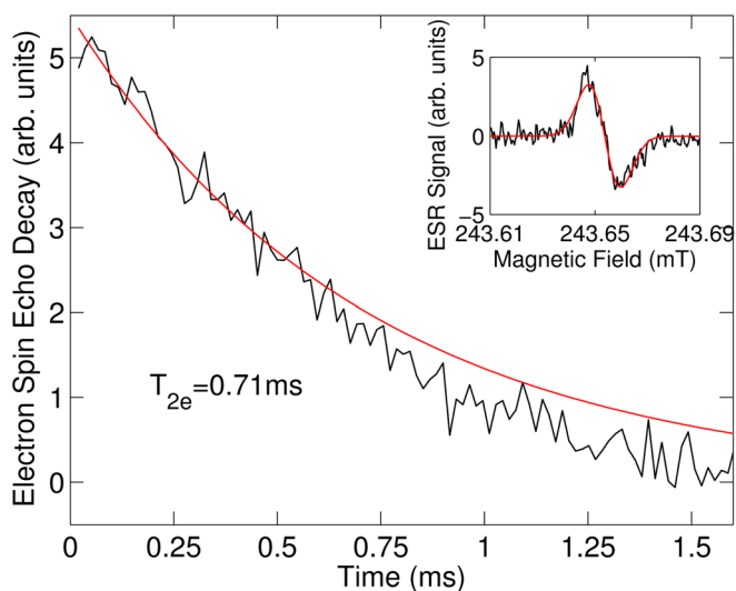
FIG. 4. ESE decay using two axis refocusing pulses (XYXY) measured at the m_l = -1/2 line of ^{28}\text{Si}:\text{Bi} at T = 8 K. The decay signal at times longer than 0.5 ms is distorted by the phase noise resulting from magnetic field fluctuations, 29 and therefore only the initial portion of the decay is used in an exponential fit to extract the electron spin coherence time of T_{2e} = 0.71 \pm 0.08 ms. The inset displays a cw-ESR spectrum of the m_l = -1/2 line and its fit yields a peak-to-peak line-width of 12.2 \pm 0.4 \mu\text{T} .
