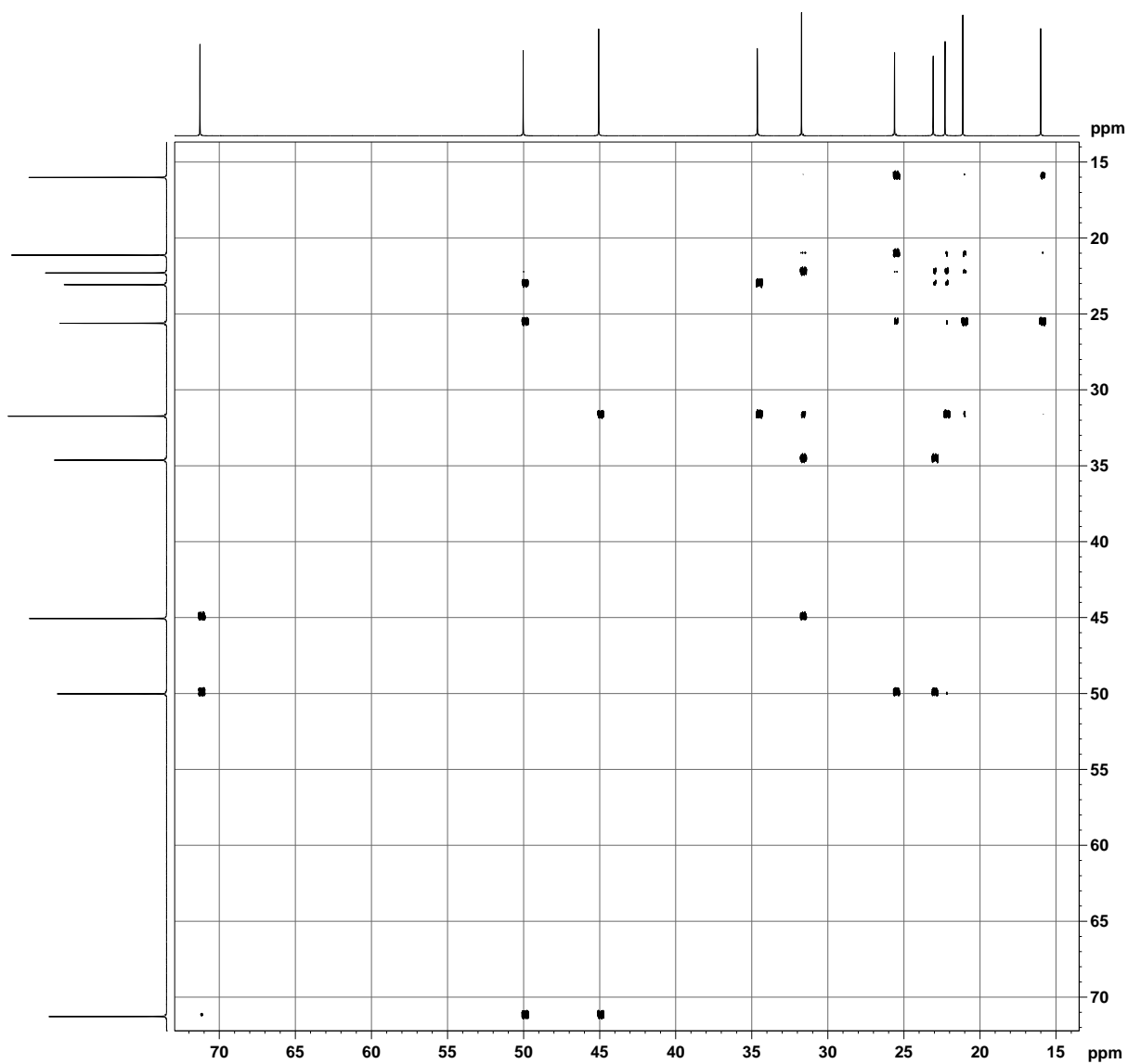
2D INADEQUATE spectrum of L-menthol in CDCl 3
