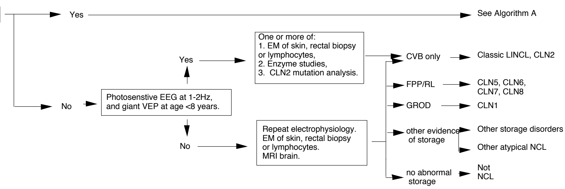
Algorithm B
