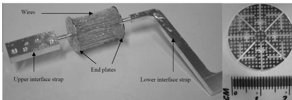
Fig. 11. Left: prototype CPA pill thermal bus. Right: end plate with 252 holes on 1.2 mm pitch.
