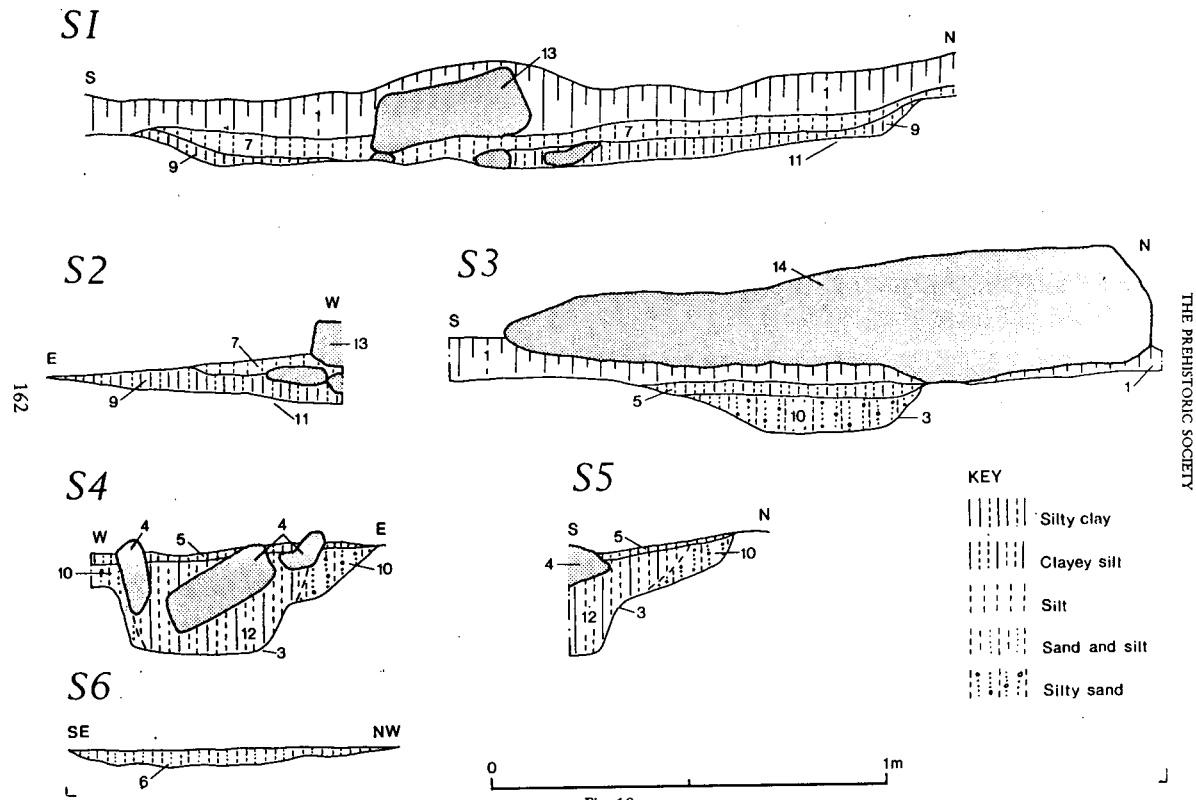
Fig. 10 Leskernick stone row terminal: sections. See Fig. 9 for locations
