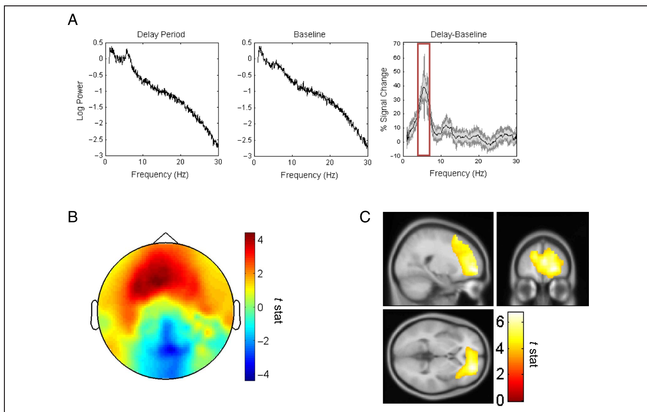
Figure 3. Delay versus baseline period, 4- to 7-Hz theta power changes. (A) Power spectra from a virtual electrode placed in the frontal midline region identified by a previous study ( x = 0, y = 58, z = 22 ; Kaplan et al., 2014) for the delay and baseline periods as well as the difference in power between the two, averaged across all trials and participants. The power difference plot shows mean \pm SEM across participants in gray. The power difference spectra show a single prominent peak at \sim 5.5 Hz, and we focus our subsequent analyses on a 3-Hz frequency band centered on this peak (i.e., 4–7 Hz). (B) Scalp level delay versus baseline period, 4- to 7-Hz theta power changes, which show an increase across the frontal midline region. (C, left) mPFC ( x = 22, y = 50, z = 0 ; z score = 4.51; peak voxel FWE corrected for the whole-brain volume, p = .012 ) theta power changes between the baseline and delay periods. Image shown at p < .001 uncorrected and overlaid on the canonical Montreal Neurological Institute 152 T1 image.
