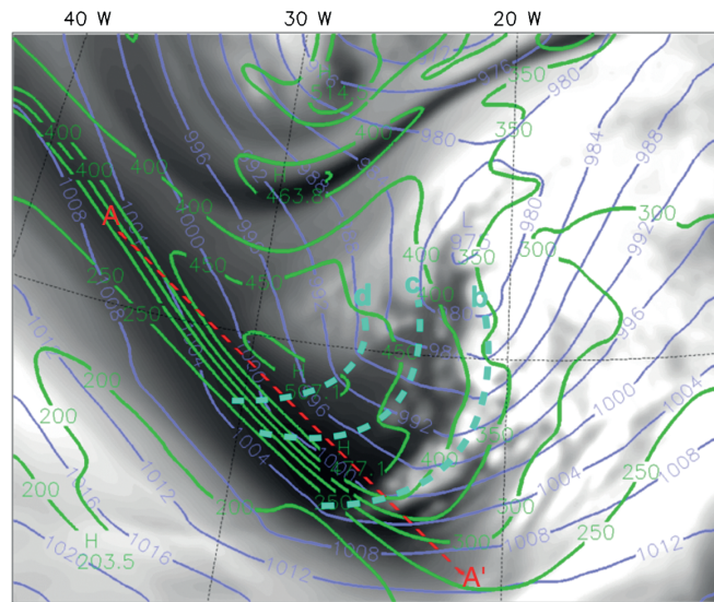
Figure 4. WRF model forecast for 2300 UTC on 5 February 2016 ( T + 17h ). Mean sea-level pressure is shown by the blue contours at intervals of 4hPa. The shading represents simulated WV channel imagery (white – moist mid-troposphere). Green contours show the height of the tropopause ( PV = 2 ) at intervals of 50hPa. Dashed cyan lines represent cold fronts and the labels 'b', 'c' and 'd' correspond to the positions of the cloud heads developing at the northern ends of these fronts. The dashed red line shows the position of cross-section AA'.
