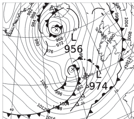
Figure 1. Met Office surface analysis valid at 0000 UTC on 6 February 2016. (Source: UK Met Office.)
