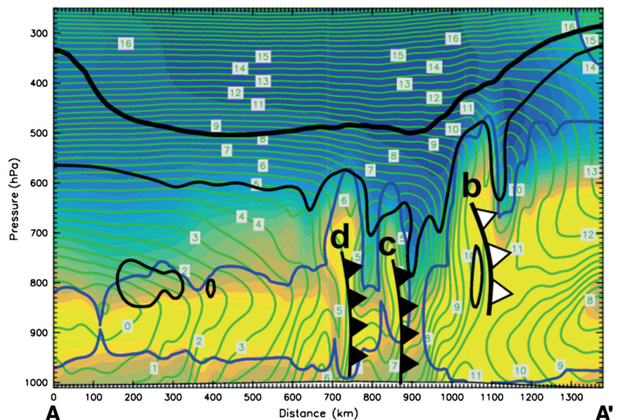
Figure 5. WRF model cross-section along AA' in Figure 4. Shading represents relative humidity from <10% (dark blue) to >90% (yellow). The thick blue contour shows where the cloud mixing ratio exceeds 0.001\text{kg}^{-1} . The tropopause ( PV = 2 ) is shown by the bold black line; the thinner black line corresponds to PV = 1 . Green contours represent isopleths of wet-bulb potential temperature at intervals of 0.5 degC. Fronts 'b', 'c' and 'd' are denoted by cold-frontal symbols. Note that front 'b' is depicted as an upper cold front.
