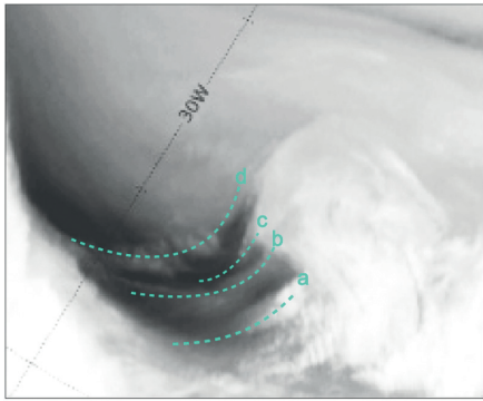
Figure 3. Meteosat water vapour image for 1900 UTC, 5 February 2016. The cold fronts are highlighted as in Figure 2(a). (Source: EUMETSAT.)
