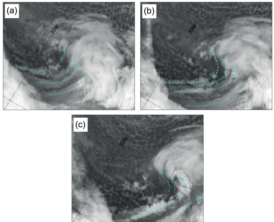
Figure 2. Sequence of Meteosat infra-red images at (a) 1900, (b) 2100 and (c) 2300 UTC on 5 February 2016. Cloud bands associated with a sequence of cold fronts are highlighted by dashed lines, labelled 'a', 'b', 'c' and 'd'. (Source: EUMETSAT.)
