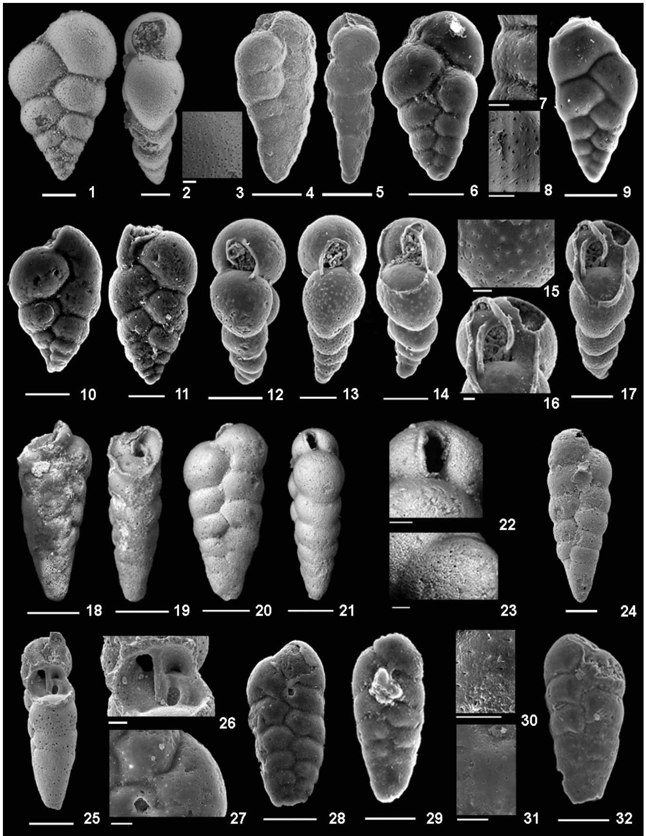
PLATE 19.1 1-17, Streptochilus martini (Pijpers, 1933); 18-32 Streptochilus pristinum Brönnimann and Resig, 1971. 499
