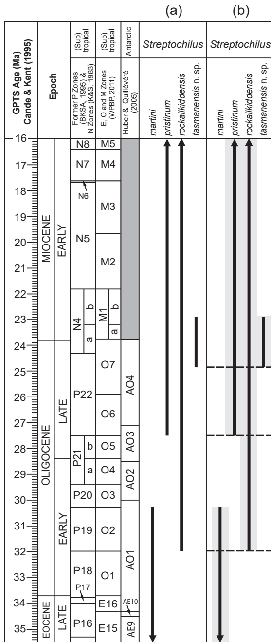
FIGURE 19.1(a) Stratigraphic ranges, and (b) phylogeny of Oligocene species of Streptochilus discussed in this chapter. Shaded vertical lines in (b) represent multiple expatriation events from the coastal benthos to the pelagic zone. Horizontal dashed lines in (b) represent first expatriation events from the coastal benthos to the pelagic zone. BKSA, 1995 = Berggren and others, 1995; K&S, 1983 = Kennett and Srinivasan, 1983; WBPB, 2011 = Wade and others, 2011.
