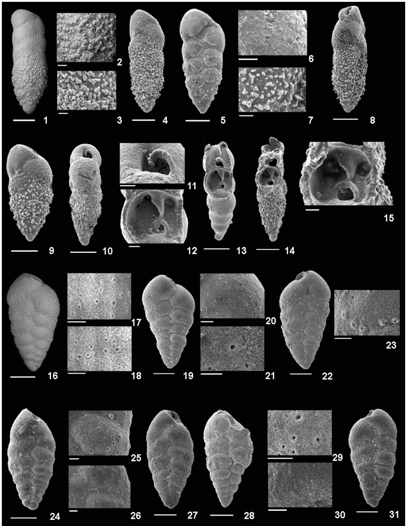
PLATE 19.2 1-15 Streptochilus rockallkiddensis Smart and Thomas, 2007; 16-31 Streptochilus tasmanensis Smart and Thomas, new species 503
