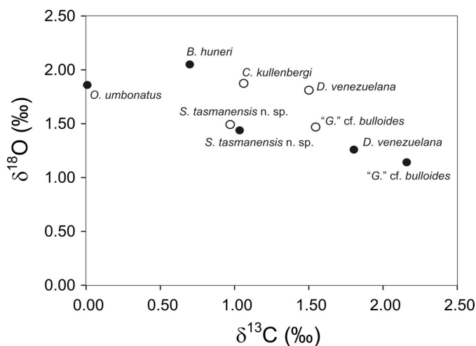
FIGURE 19.2 Oxygen and carbon isotope values (‰) of late Oligocene Streptochilus tasmanensis n. sp., Dentoglobigerina venezuelana , " Globigerina " cf. bulloides , Cibicidoides kullenbergi , Oridorsalis umbonatus and Bolivina huneri for samples ODP Hole 1170A/43X/3, 56-57 cm (solid black circles) and ODP Hole 1170A/43X/5, 57-58 cm (open black circles).
