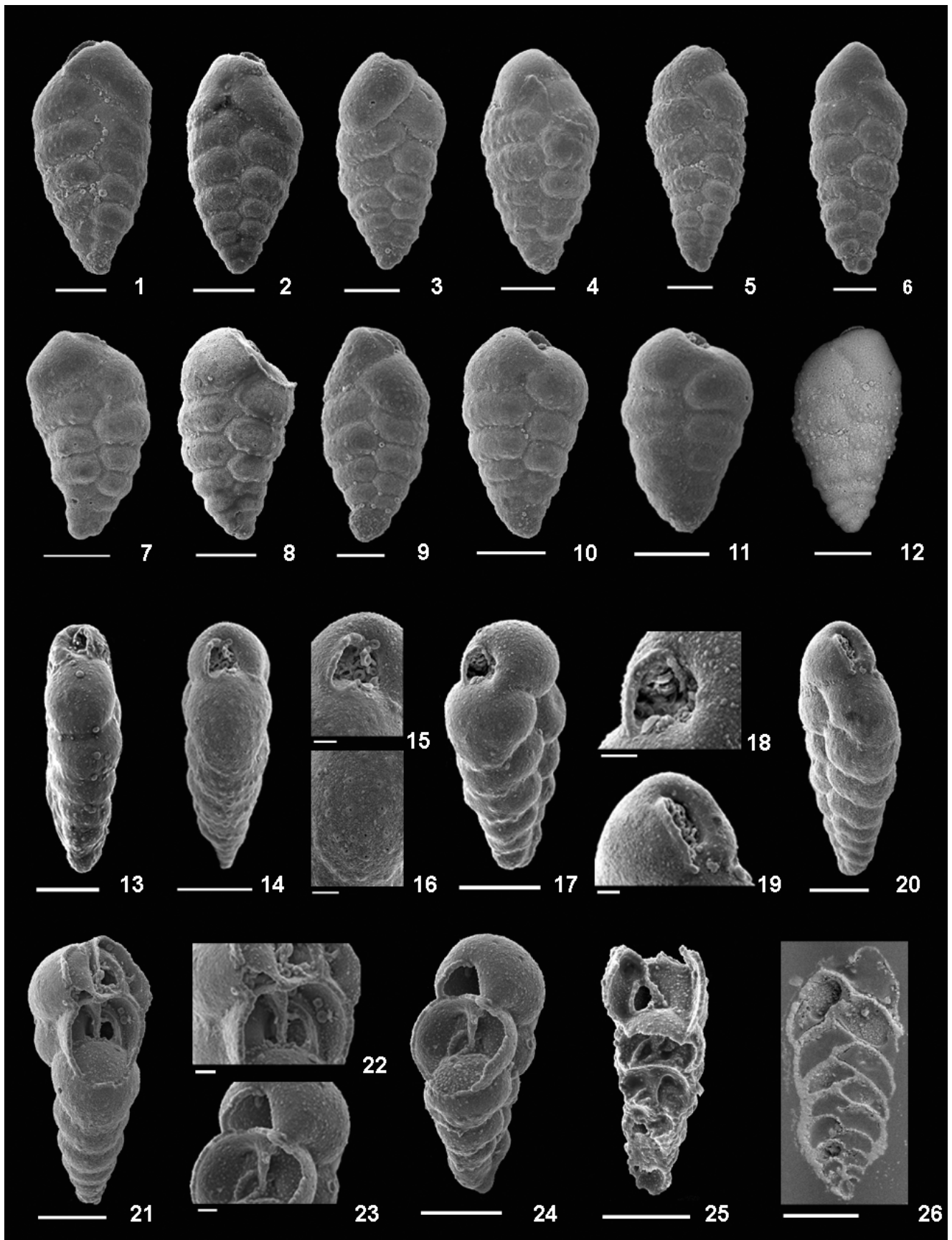
PLATE 19.3 Streptochilus tasmanensis Smart and Thomas, new species
