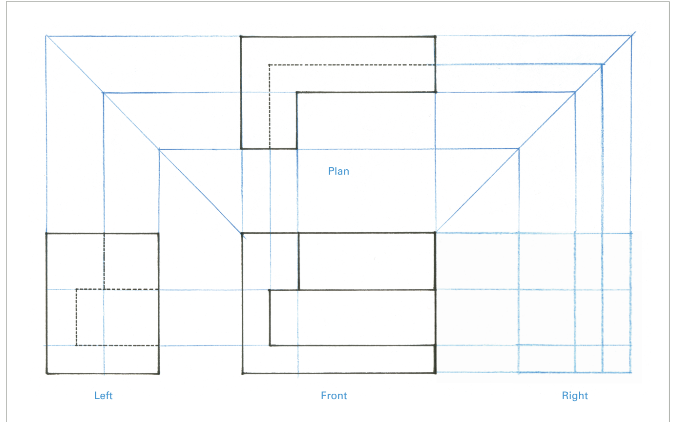
6.2b Third Angle Projection
