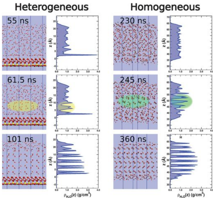
Fig. 3 Snapshots and water density profiles for a homogeneous (right) and heterogeneous (left) nucleation event. In the presence of kaolinite, the supercooled water (55 ns) has a high density peak corresponding to the first contact layer. There is also a noticeable second peak, but this is far less intense and much broader. After 61.5 ns, nucleation has started. There is a slight reduction in density of the first density peak, but this is still much higher than anywhere else in the system. Rearrangement of water molecules in the second layer associated with a split in the density peak (highlighted in yellow), is also seen and is indicative of an ice-like layer forming. By 101 ns the first contact layer has fully transformed to ice and the density is similar to that observed in the rest of the system. Note that it is the prism face of ice exposed to the kaolinite surface and that we only observe hexagonal ice. In contrast, for the homogeneous slab we see a fairly uniform density profile in the supercooled regime (230 ns). We also see a mixture of hexagonal and cubic stacking. In this instance, the initial nucleation event (highlighted in green) leads to a cubic stacking arrangement. The densities are averages over a 2.5 ns interval centred at the specified time. The colour scheme is the same as Fig. 1.
