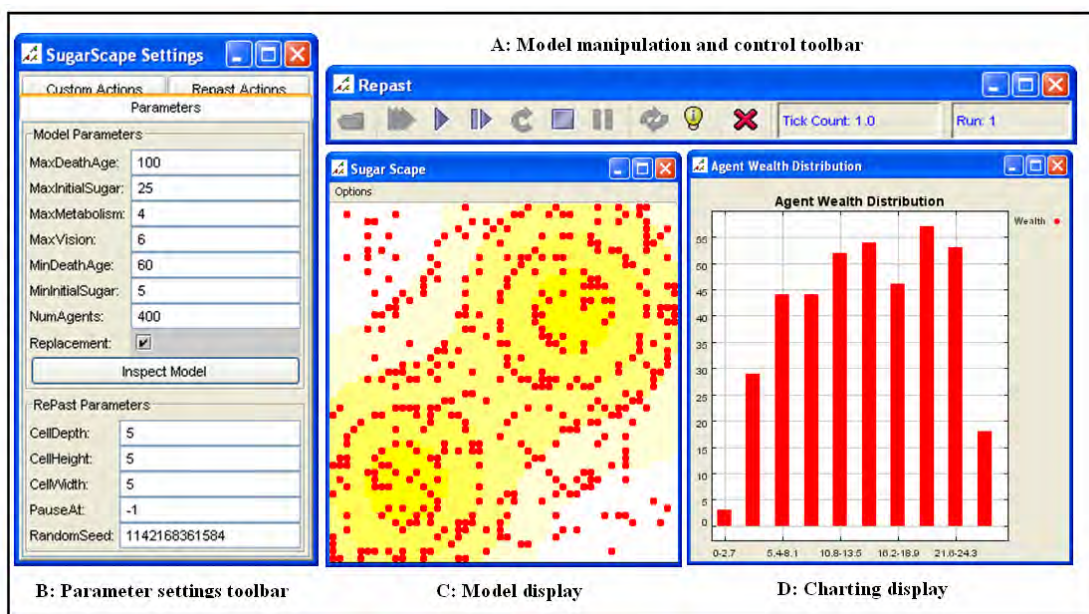
Figure 1: A typical selection of Repast toolbars and displays used during a run of the Sugarscape model.
