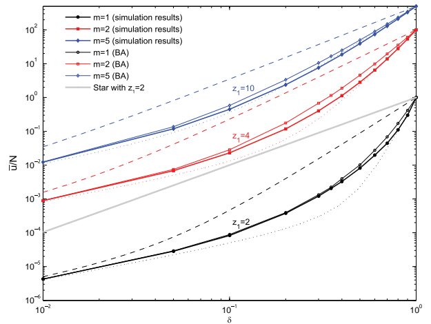
FIG. 3: Average utility for the simulation results (solid curve and symbols) and the BA model (solid curve, open symbols) for m = 1 ( z_1 = 2 ), 2 ( z_1 = 4 ) and 5 ( z_1 = 10 ). We also plot the analytical curves for average utility in Poisson (dotted curve) and scale-free (dashed curve) networks for z_1 = 2, 4 and 10 and \gamma = 3.1 (for scale-free networks). Curves were computed for networks with N = 5 \times 10^3 vertices and have been shifted vertically for distinct values of z_1 . The curve in gray is the average utility of a star with N = 5 \times 10^3 and z_1 \approx 2 . Simulation results were averaged over 30 runs.
