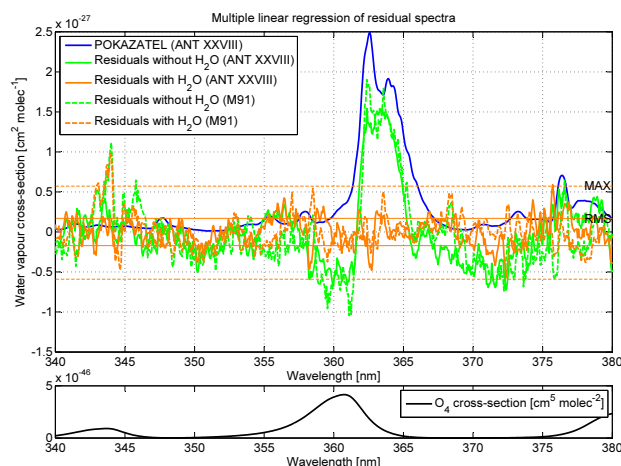
Figure 10. Using a multi-linear regression on the residual spectra from the campaigns ANT XXVIII/1-2 and M91 , the water vapour dSCD-correlated residual structures were obtained. Negative values can be explained by compensation of the missing water vapour absorption structures by other absorbers included in the DOAS fit. The resulting spectrum including water vapour absorption yields an estimate on the accuracy of the convolved cross-section.
