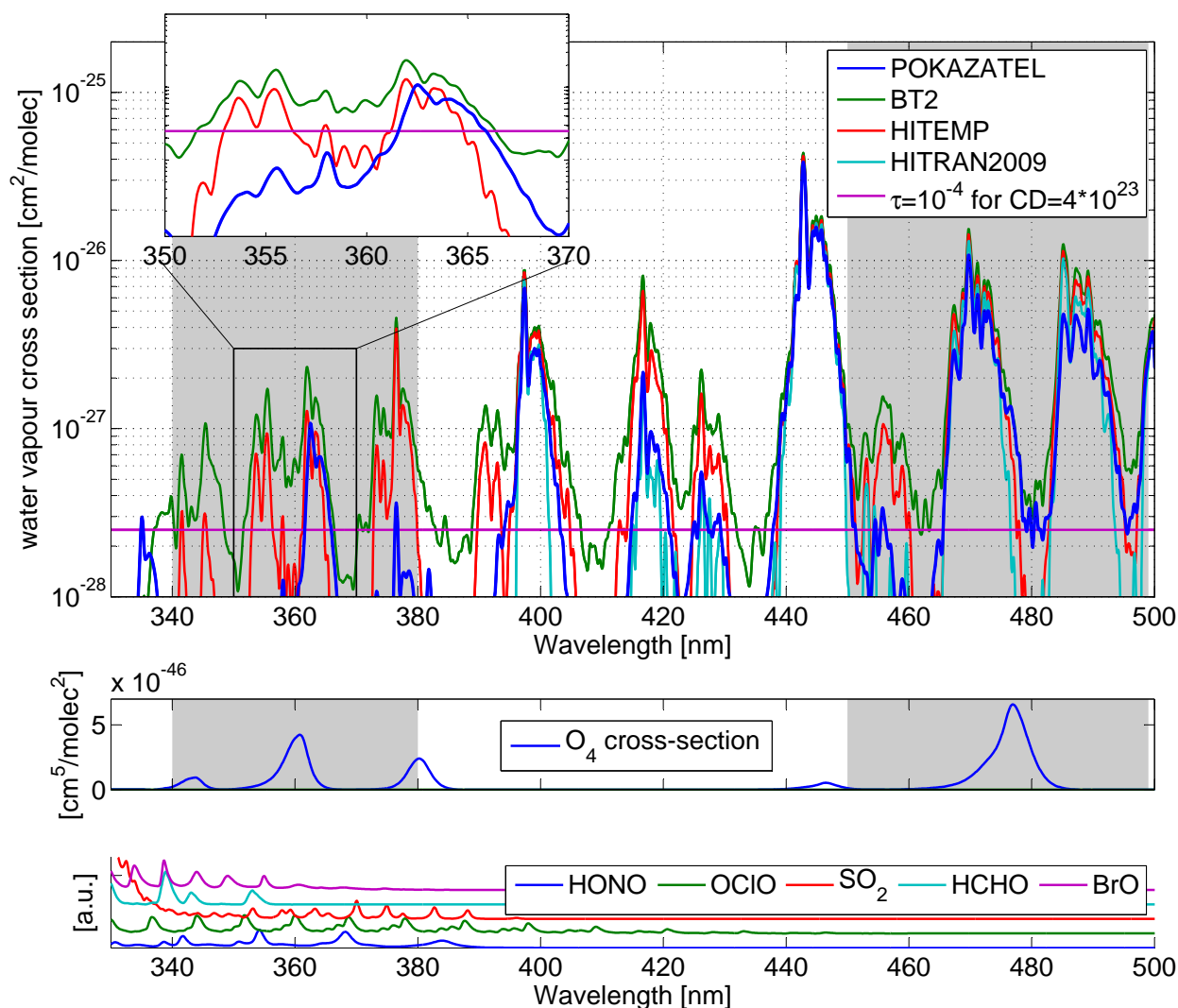
Figure 1. Overview of some recently published water vapour cross-sections convoluted to a spectral resolution of 0.5 nm in the spectral interval from 330 to 500 nm. Also indicated is a typical MAX-DOAS detection limit for a differential OD of 10^{-4} at a water vapour column density of 4 \cdot 10^{23} molec \text{cm}^{-2} (purple line, top panel). The middle panels shows the \text{O}_4 absorption cross-section, the lowermost panel other absorbers of atmospheric relevance (HONO, OCIO, \text{SO}_2 , HCHO, and BrO) in this spectral range.
