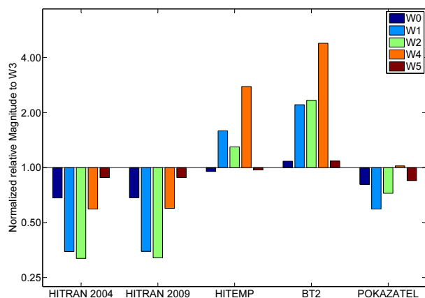
Figure 11. Comparison of different available water vapour cross-section data in the blue spectral range using the different band listed in Table 6. W3 was used as a respective reference in all cases and is therefore by definition unity. All magnitudes were normalized with respect to the rescaled HITEMP absorption cross-section from Lampel et al. (2015b) to obtain relative magnitudes of each of the absorption bands W0, W1, W2, W4 and W5. A value of '1' identifies good agreement with the relative magnitude of the absorption bands' sizes according to MAX-DOAS and LP-DOAS measurements presented in Lampel et al. (2015b).
