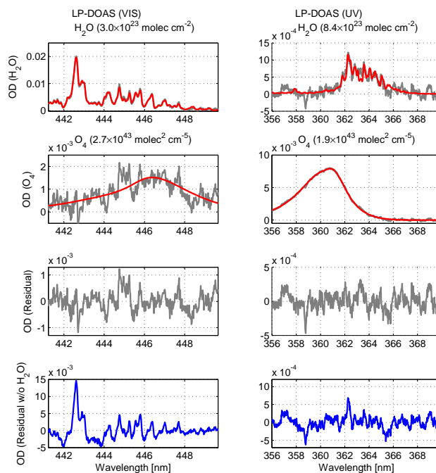
Figure 3. A LP-DOAS fit result for the fitting intervals around 363 and 442 nm. The spectra were recorded on August 29th, 2015 between 20:58 and 21:45 UTC. Top left panel: At 442 nm the \text{H}_2\text{O} dSCD (3.0 \pm 0.04) \times 10^{23} \text{ molec cm}^{-2} ( \text{O}_4 dSCD (2.7 \pm 0.6) \times 10^{43} \text{ molec}^2 \text{ cm}^{-5} ). Top right panel: At 360 nm the \text{H}_2\text{O} dSCD (8.4 \pm 0.6) \times 10^{23} \text{ molec cm}^{-2} ( \text{O}_4 dSCD (1.85 \pm 0.03) \times 10^{43} \text{ molec}^2 \text{ cm}^{-5} ).
