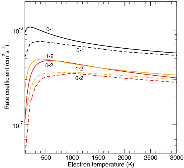
Figure 2. Rate coefficients for rotational excitation of \text{HeH}^+ from Rabadán et al. (1998) (—) against our results (---).
