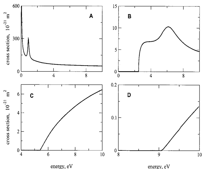
Fig. 12. Total elastic cross sections for electron scattering off CF_2 (A); electron impact excitation cross sections for the excitation of the metastable {}^3B_1 state (B), bound and radiative {}^1B_1 state (C) and other dissociative {}^3A_2 , {}^1A_2 and {}^3B_2 states (D).
