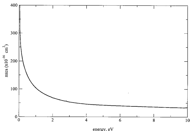
FIG. 16. Momentum transfer cross section for electron scattering by the \text{CF}_3 radical.
