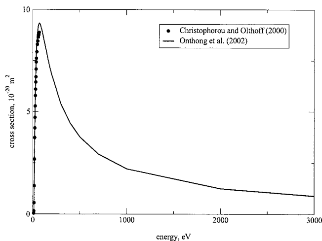
FIG. 4. Ionization cross sections for \text{CF}_3\text{I} .
