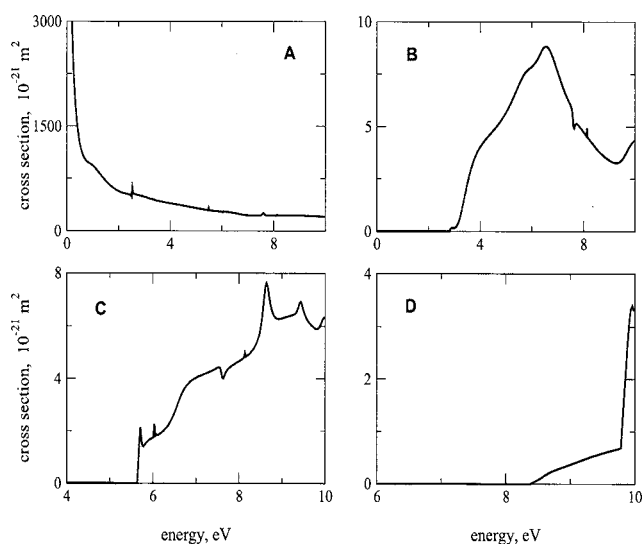
Fig. 10. Total elastic cross sections for electron scattering off CF (A); and electron impact excitation cross sections for the excitation of the metastable a ^4\Sigma^- state (B), dissociative A^2\Sigma^+ and B^2\Delta states (C) and other states C^2\Sigma^- and b^4\Pi (D).
