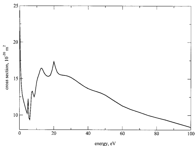
FIG. 6. Momentum transfer cross section for \text{C}_2\text{F}_4 (Winstead and McKoy 26 ).
