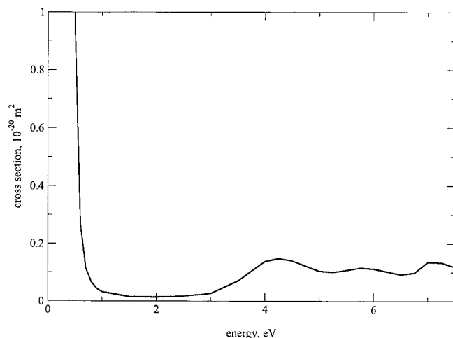
FIG. 5. Electron attachment cross section for \text{CF}_3\text{I} (Christophorou and Olthoff 14 ).
