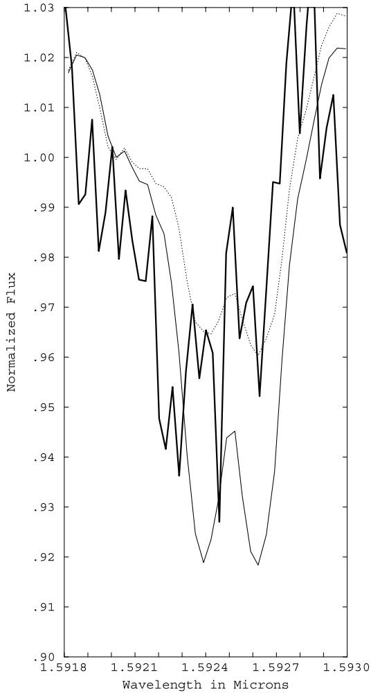
Figure 6. Spectrum for CM Dra compared with synthetic spectra for specific features of interest. Thick continuous line: CM Dra; thin continuous line: 3100 K, [M/H] = -1.0 model; dotted line: 3300 K, [M/H] = -1.0 model. The atomic feature is Si I ( \sim 1.5931 \mu\text{m} shifted to \sim 1.5925 \mu\text{m} ).
