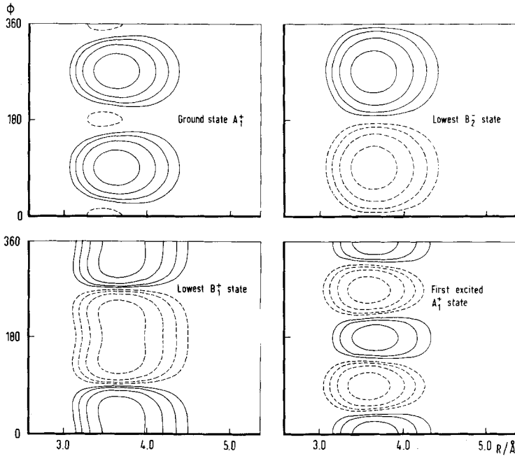
Figure 1. Cuts through the vibrational ( J = 0 ) wave functions in (N_2)_2 for the lowest four states, with \theta_A and \theta_B fixed at 90^\circ . The contours enclose regions with 8%, 16%, 32%, and 64% of the maximum amplitude. Solid curves correspond with positive values of the wavefunction and dashed curves with negative values.
