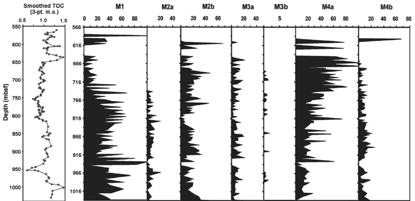
TEXT-FIGURE 5 Relative distribution (in percentage) of agglutinated foraminiferal morphotypes in Hole 909C (566.97-1040.71 mbsf). Also shown is the 3-point moving average of percent Total Organic Carbon values in the studied section (data from Stein and Stax 1996).
