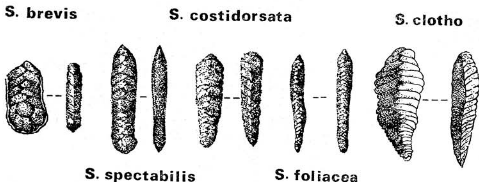
Fig. 1. Five species of Spiroplecta described by Grzybowski [redrawn after Grzybowski 1898, 1901], all considered synonymous to Spiroplectammina spectabilis in this study. Also listed are taxa placed in S. spectabilis by previous authors.
