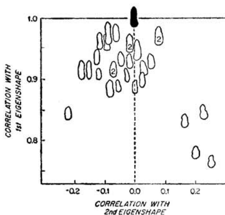
Fig. 3. Range of observed shapes from a single sample from Biecz arranged according to shape, with hypothetical first eigenshape (figure in black). The number (2) inside a shape indicates overlapping specimens
