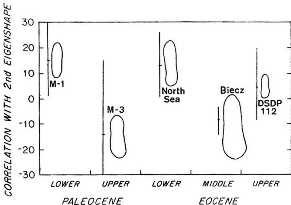
Fig. 4. Correlation of the first eigenshapes of the within-sample eigenshape analysis (average shape of each sample) with the second eigenshape of the between-sample eigenshape analysis. Lines represent 95% confidence intervals of the correlation of observed shapes with the second eigenshape of each sample.
