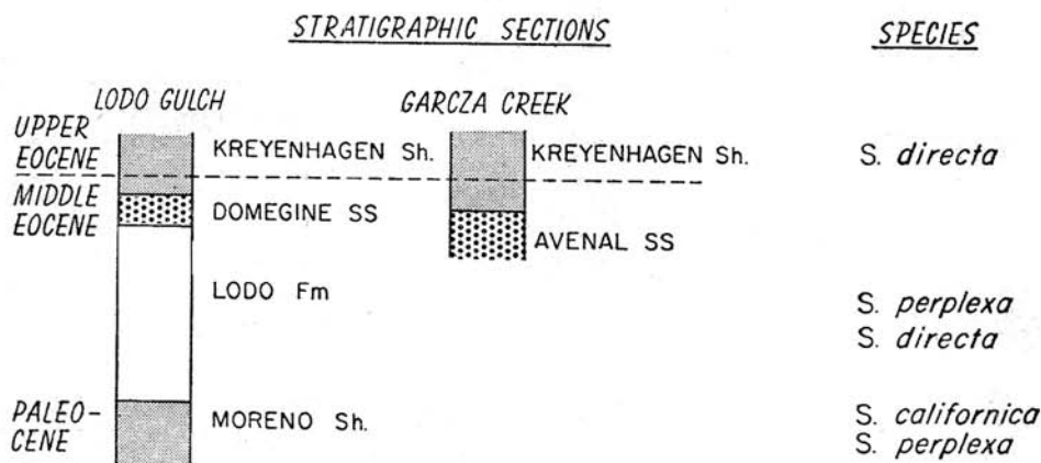
Fig. 2. Stratigraphy of the Californian type formations for S. californica , S. directa and S. perplexa , after Poore (1976).
