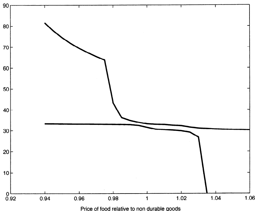
FIGURE 15. E-bounds to demand responses.
