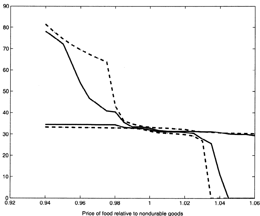
FIGURE 19. Improved E-bounds on demand responses.
