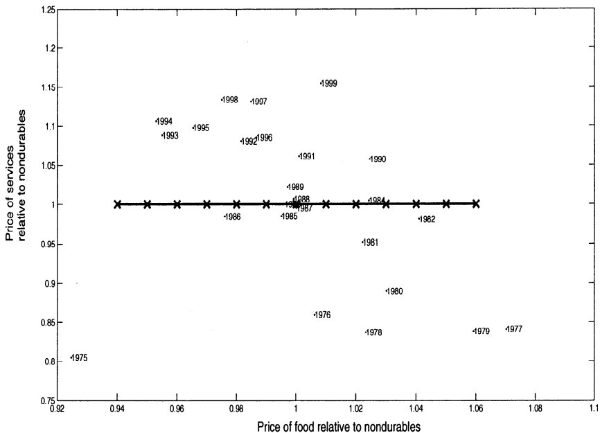
FIGURE 11. The times series of relative prices.
