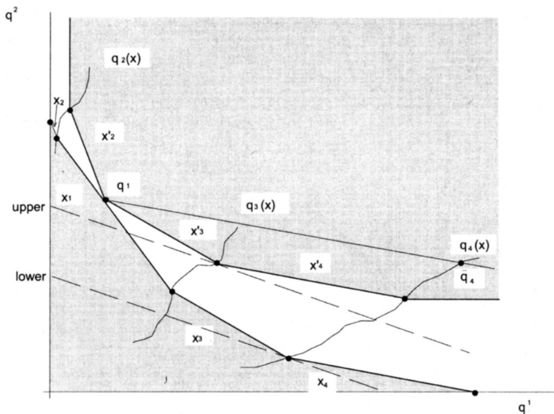
FIGURE 16. Bounds on the cost-of-living index using expansion paths.
