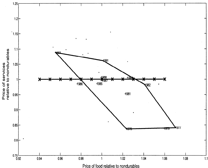
FIGURE 14. Convex hull for RP consistent comparisons.
