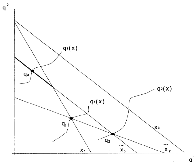
FIGURE 2. Testing GARP with expansion paths.
