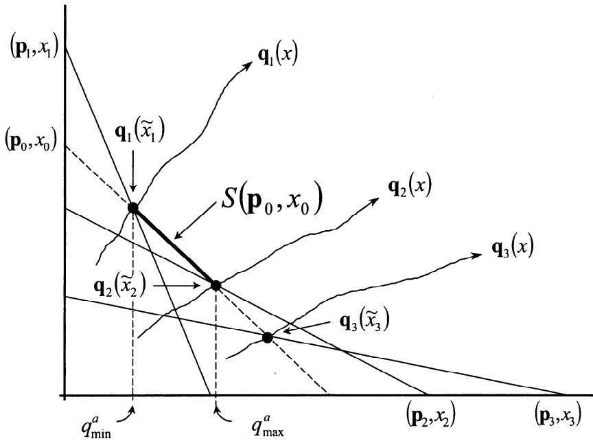
FIGURE 10. E-bounds on demand responses.
