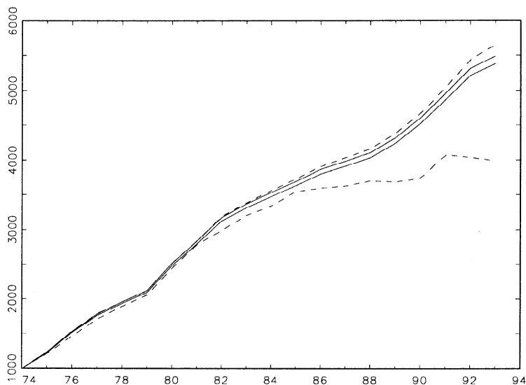
FIGURE 17. GARP bounds and classical RP bounds, 1974 to 1993.
