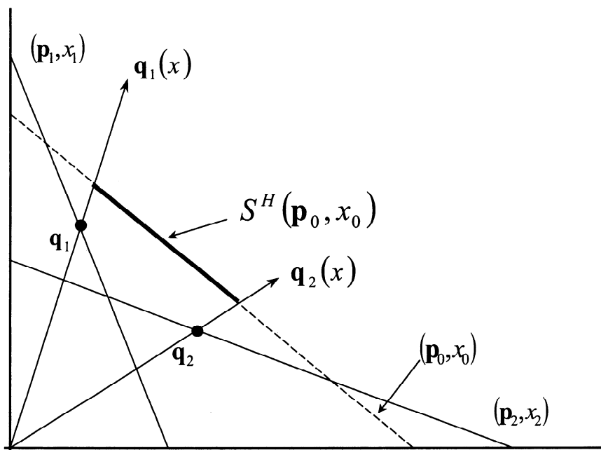
FIGURE 9. The support set under homotheticity.
