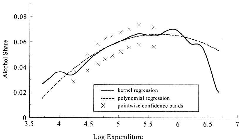
FIGURE 6. Nonparametric Engel curve: alcohol share.
