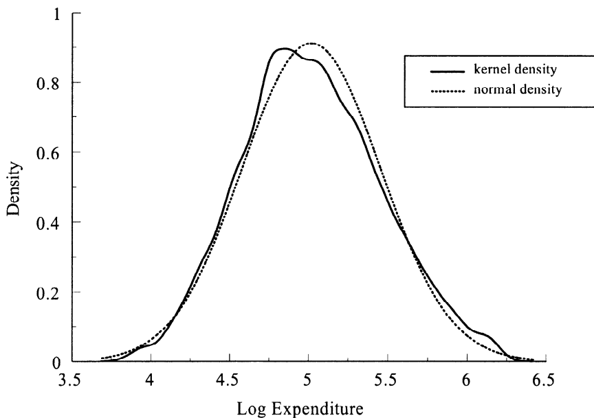
FIGURE 3. The density of log expenditure, FES 1980.
