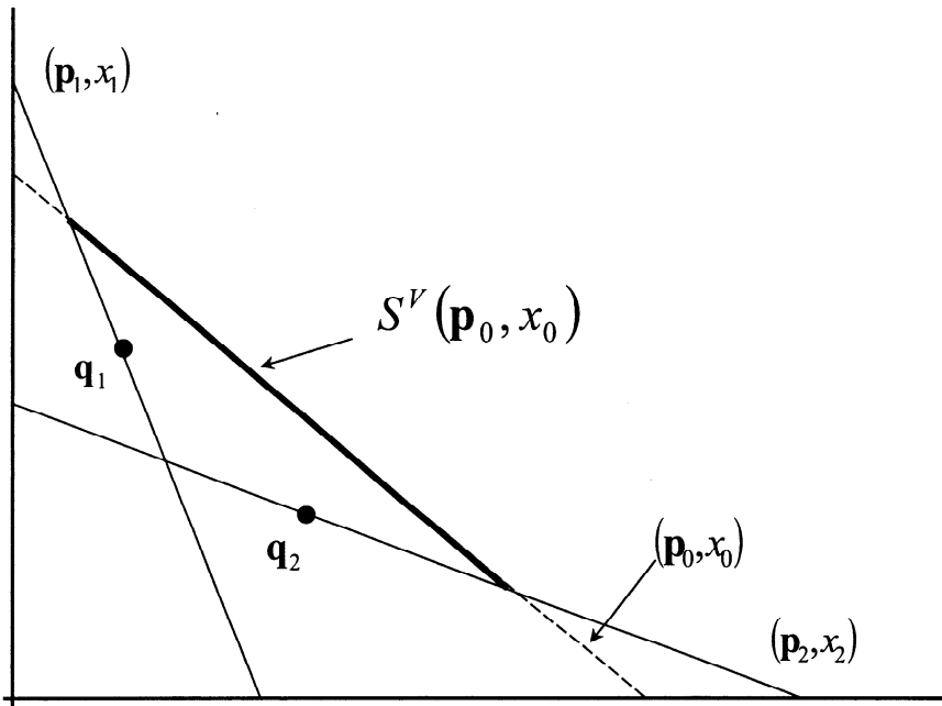
FIGURE 8. The Varian support set.
