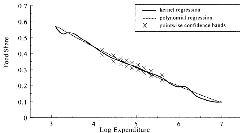
FIGURE 5. Nonparametric Engel curve: food share.
