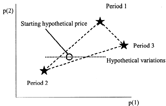
FIGURE 13. Convex hull.
