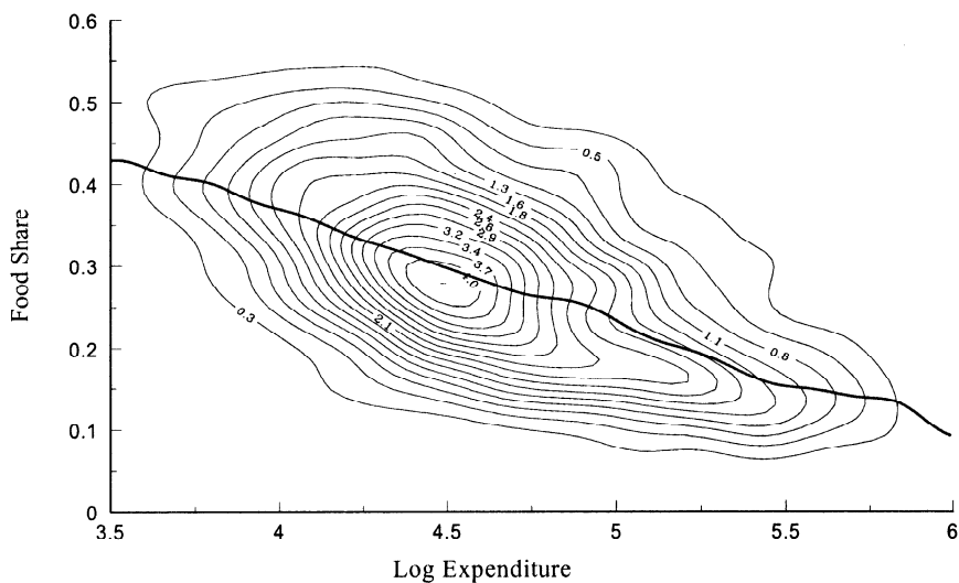
FIGURE 4. Bivariate kernel density: food share and log expenditure.
