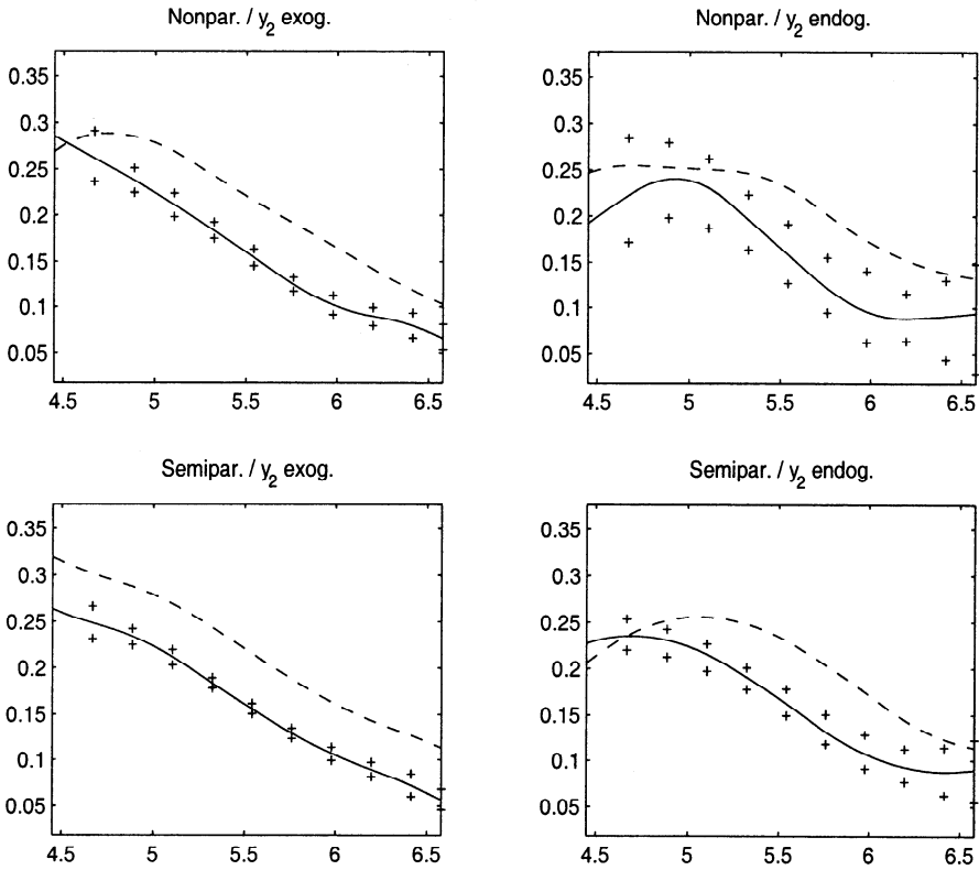
FIGURE 7. The estimated Engel curve for food:dashed curves with children; solid curves without children; plusses (+) 95% confidence bands.
