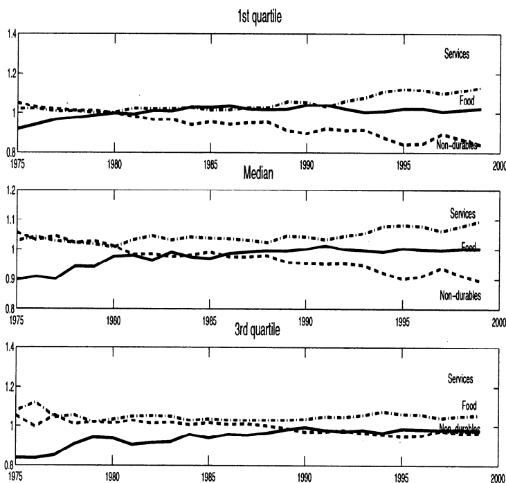
FIGURE 18. Taste changes across the income distribution.
