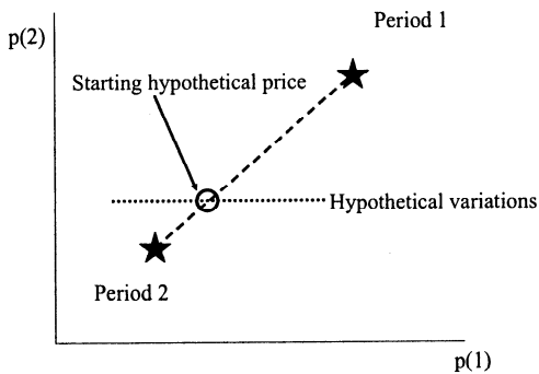
FIGURE 12. Convex combination.
